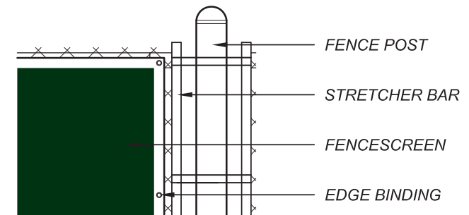
ATTACHMENT ENLARGEMENT
